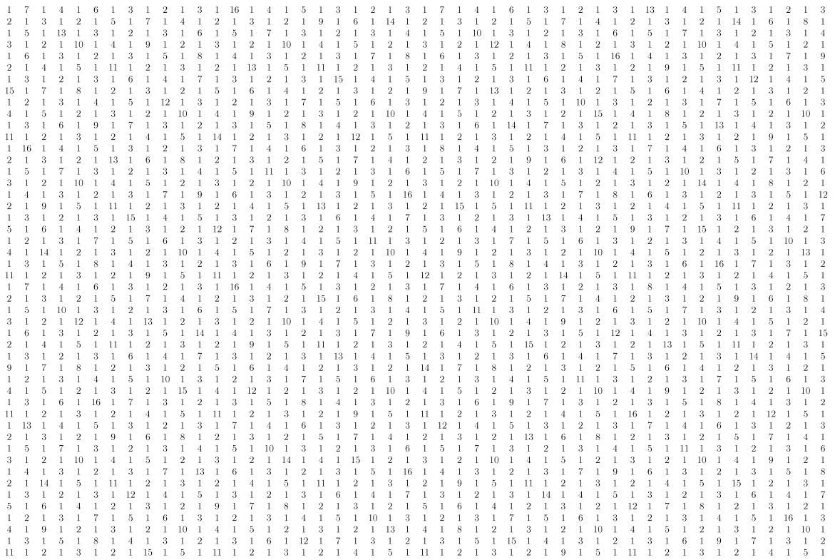
Fig. 1. Our 48 \times 48 periodic solution in 16 colours.
